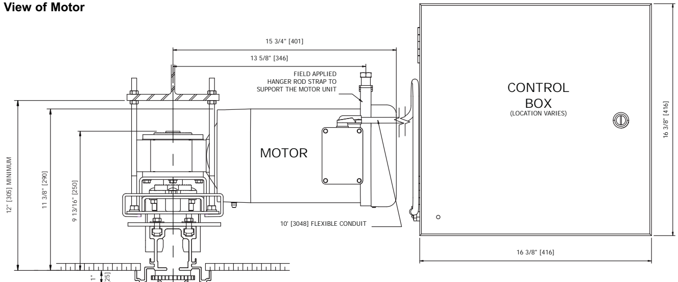
End View of Motor
